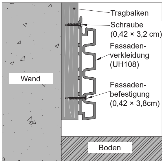
Detail B-1b
