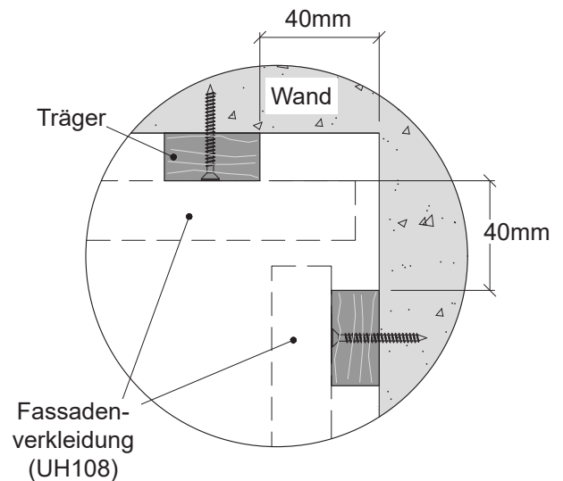
Detail 3-3
