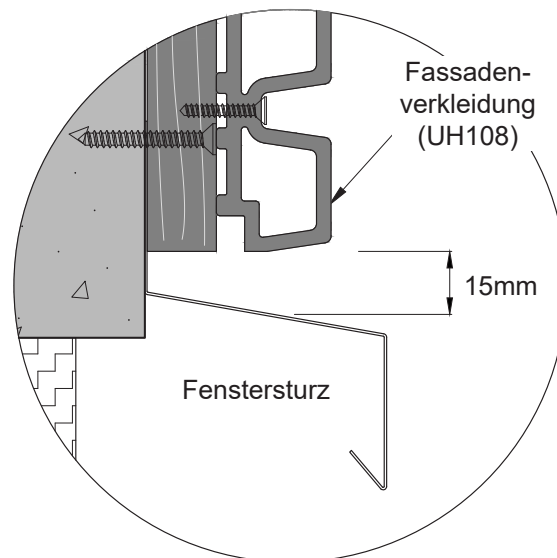
Detail 15-1
