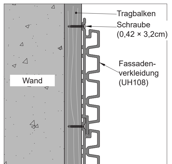
Detail C-2b
