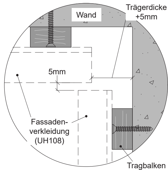
Detail 5-2
