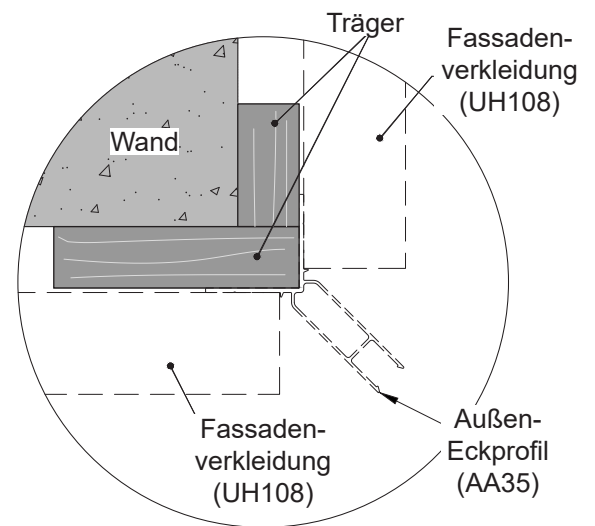
Detail 3-4
