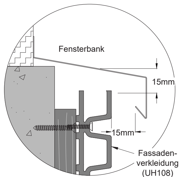
Detail 15-2
