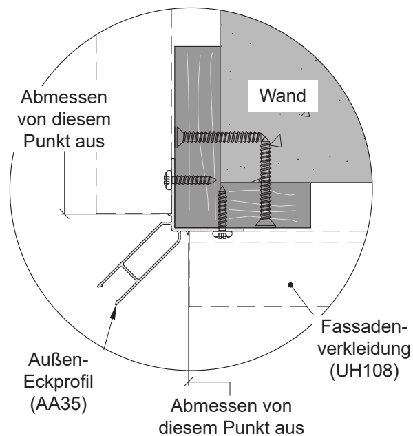
Detail 5-3
